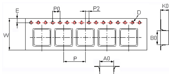
Tape Dimensions
