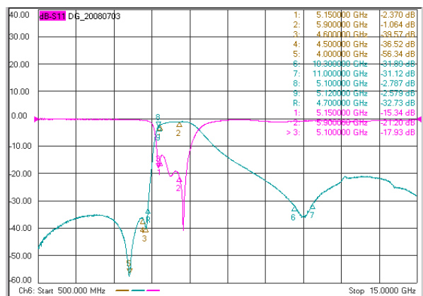
BPF2012T5500HA3
