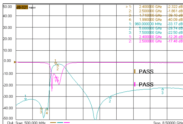
BPF2012T2450HA6
