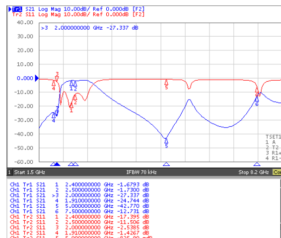
BPF2520T2450HA2
