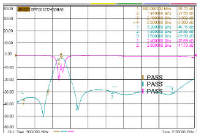
BPF2012T2450HAB
