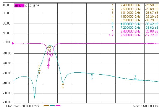
BPF2012T2450HA8
