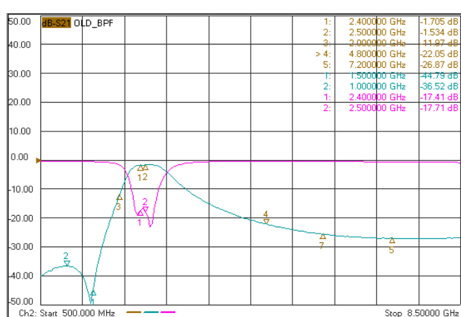
BPF1608T2450HA3
