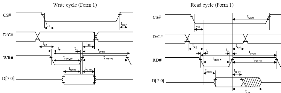
8080-series parallel interface characteristics (Form 1)
