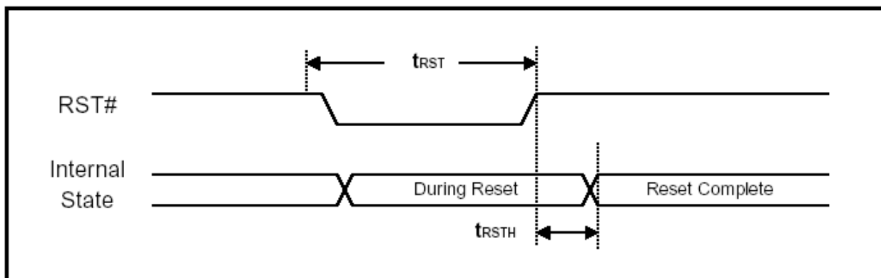
Reset timing
