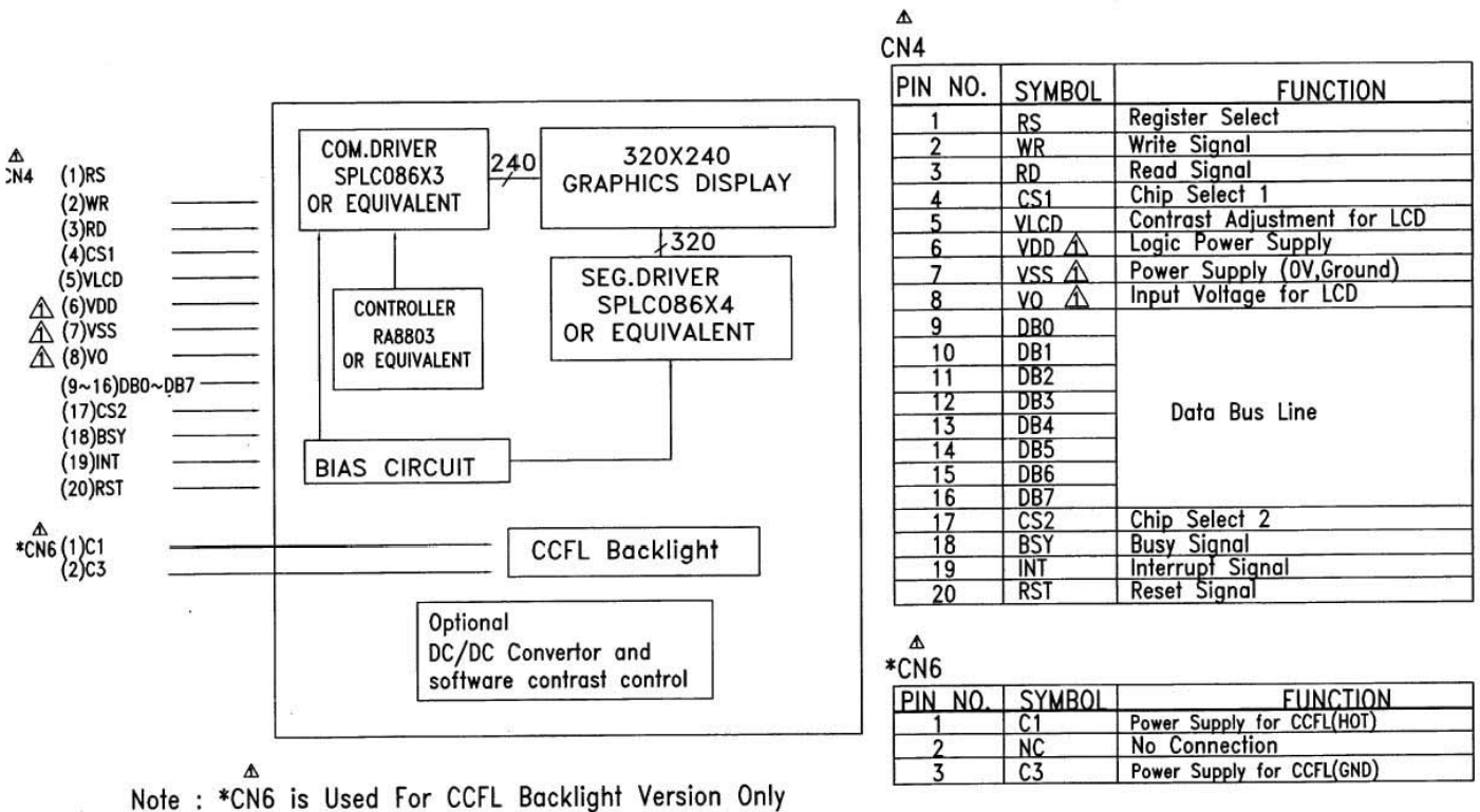
Figure2. BLOCK DIAGRAM and PIN DESCRIPTION:
