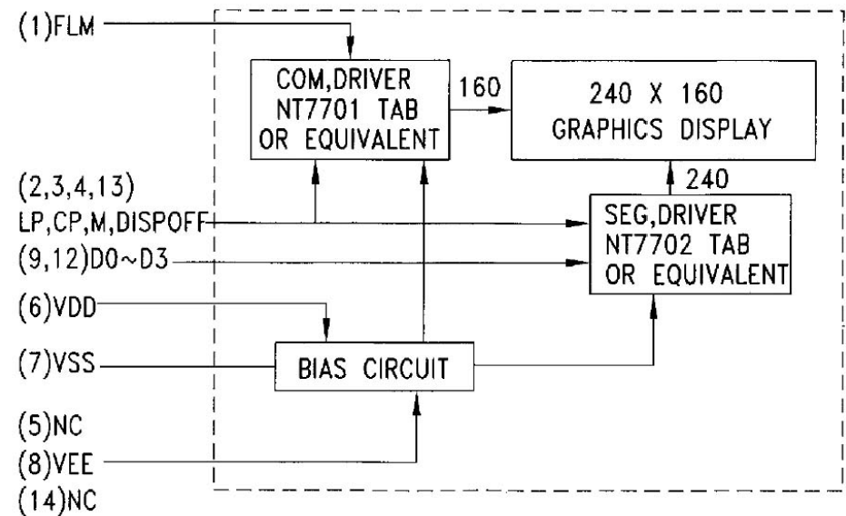
FIGURE 2. BLOCK DIAGRAM.
