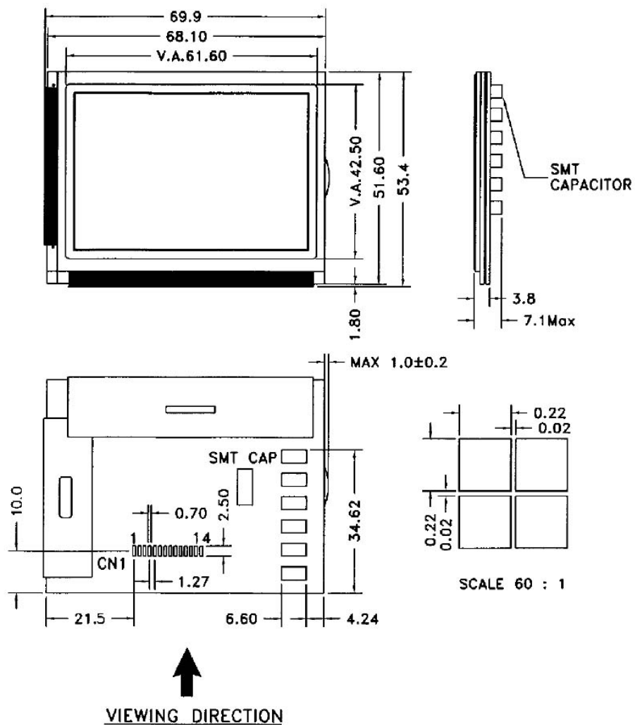
FIGURE 1. COUNTER DRAWING FOR GENERAL MODULE
