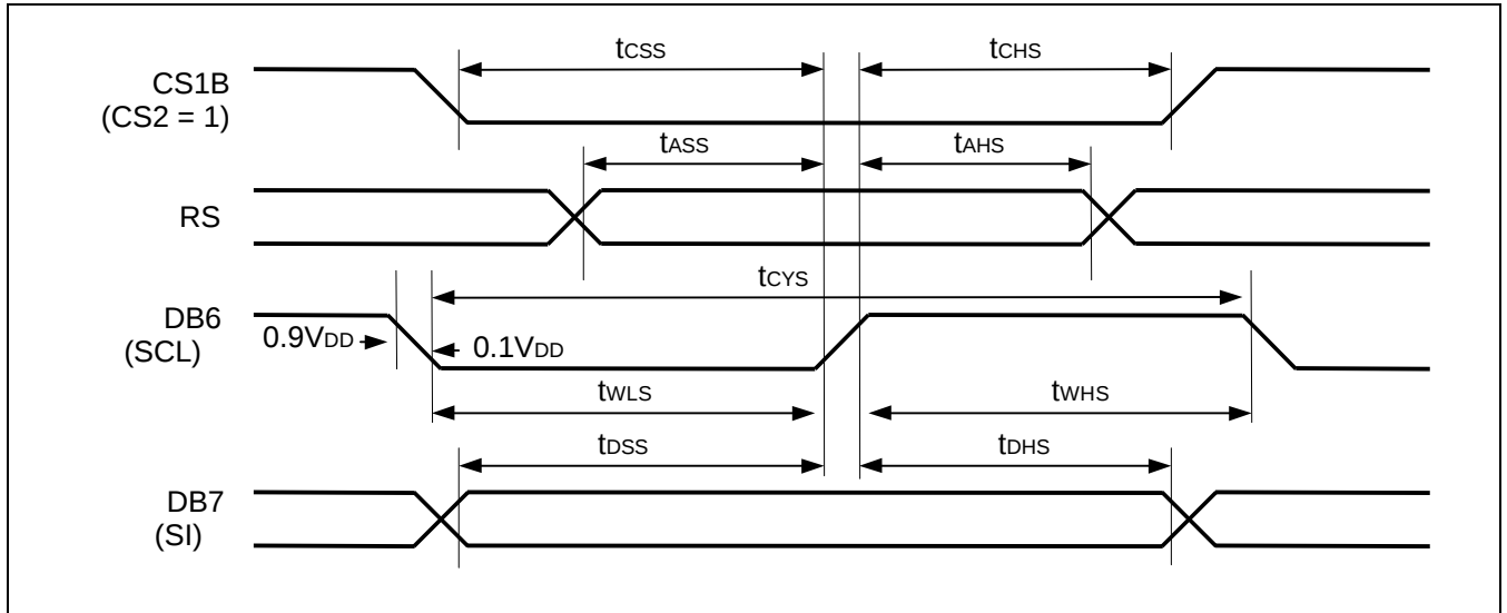
Figure . Serial Interface Characteristics
