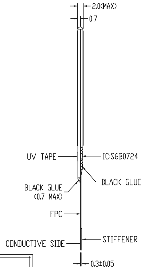
DETAIL C:
