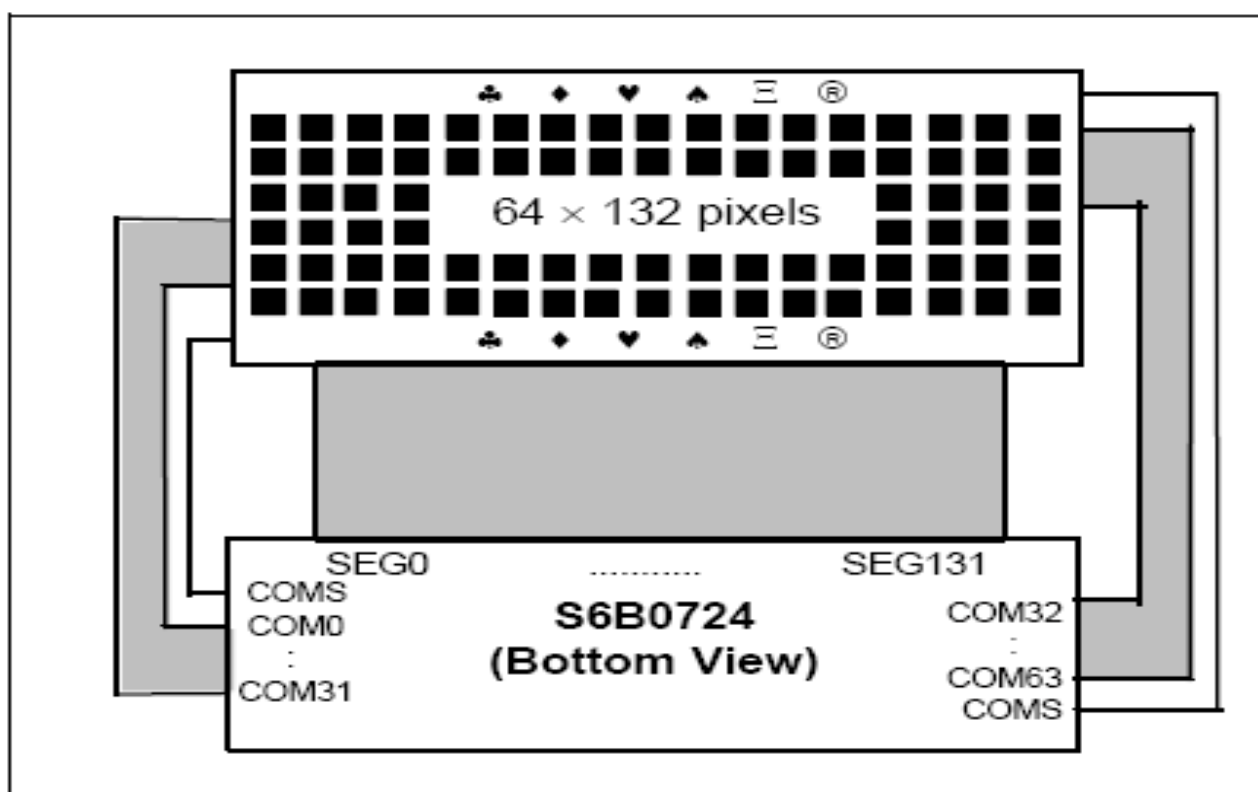
Figure 38. SHL = 1, ADC = 0
