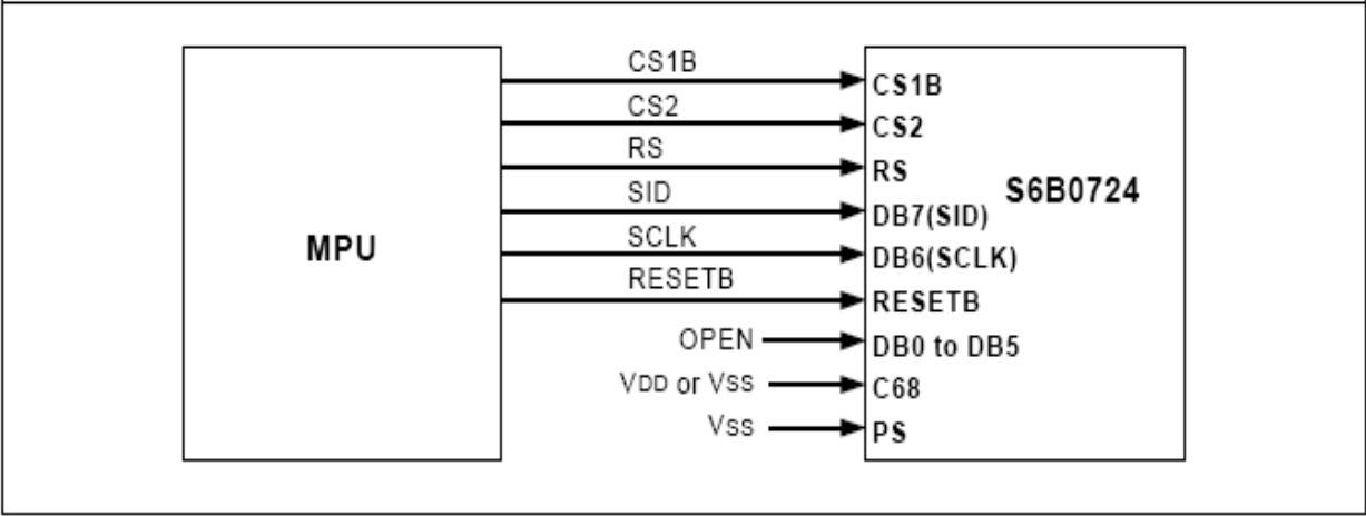
Figure 37. Serial Interface (PS = "L", C68 = "H or L")
