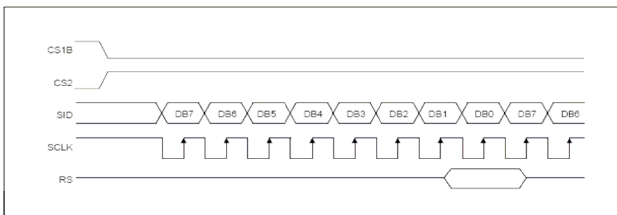
Figure 3. Serial Interface Timing
